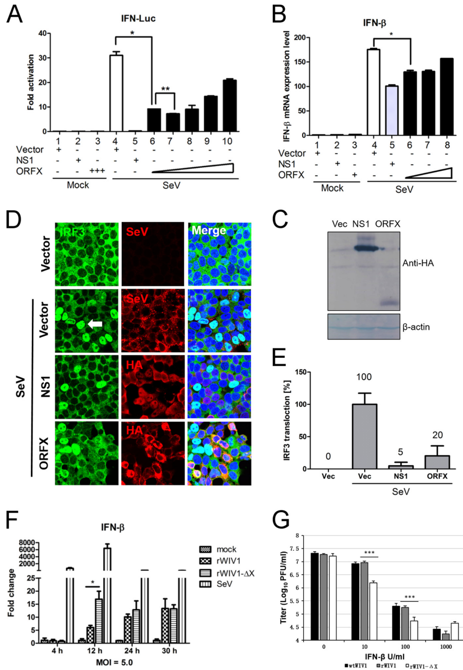
FIG 4 ORFX protein inhibits the production of type I interferon. (A and B) 293T cells seeded in 12-well plates were transfected with 100 ng pIFN- \beta -Luc, 5 ng pRL-TK, empty vector, an influenza A NS1-expressing plasmid, or increasing doses (100, 200, 400, 600, and 800 ng) of an ORFX-expressing plasmid. Empty vector was added appropriately to ensure that cells in each well were transfected with the same amount of plasmids. The cells were infected with Sendai virus (100 hemagglutinating units/ml) at 24 h posttransfection. Samples were collected at 12 h postinfection, followed by dual-luciferase assay. The results were expressed as the firefly luciferase value normalized to that of Renilla luciferase. The relative expression of IFN- \beta mRNA was determined by quantitative RT-PCR and normalized to the expression level of GAPDH mRNA. (C) The expression of the NS1 and ORFX proteins was analyzed by Western blotting with an antibody against HA tag. The experiments were replicated three times. (D and E) For the IRF3 translocation assay, 293T cells were transfected with empty vector-, NS1-, or ORFX-expressing plasmid. After 24 h, the cells were infected with Sendai virus to induce IRF3 nuclear translocation. The cells were fixed at 8 h postinfection and stained with anti-HA IgG. A goat anti-Sendai virus polyclonal IgG was used to stain the cells transfected with empty vector. A rabbit anti-IRF3 polyclonal IgG was used to label IRF3. The white arrow indicates IRF3 nuclear translocation. The relative IRF3 translocation ratios were calculated for each group by counting the number of IRF3 nuclear translocation cells (randomly selected from at least 4 fields) and dividing by the total number of infected or transfected cells. The IRF3 nuclear translocation efficiency of each group was expressed as the percentage of their relative IRF3 translocation ratios to that of the control (cells transfected with empty vector). (F) Calu-3 cells were mock infected or infected with rWIV1 or rWIV1- \Delta X (MOI of 5) or SeV (100 HAU/ml). At 4, 12, 24, and 30 h postinfection, the cell RNA was extracted and used for quantitative RT-PCR of the expression level of IFN- \beta mRNA. The experiment was performed in triplicate and replicated twice. (G) Vero E6 cells were pretreated with indicated amount of IFN- \beta , infected with wtWIV1, rWIV1, or rWIV1- \Delta X at an MOI of 0.1 PFU/cell, and posttreated with IFN- \beta . Viral replication was analyzed at 24 h postinfection by plaque assay. The experiment was performed in triplicate and replicated twice. The differences between selected groups were significant, with P values of less than 0.05, as follows: 0.0049 (*; bars 4 and 6 in panel A), 0.0008 (**; bars 6 and 7 in panel A), 0.0072 (*; bars 4 and 6 in panel B), 0.018 (*; bars for rWIV1 and rWIV1- \Delta X in panel F), and <0.0001 (***) in panel G).
